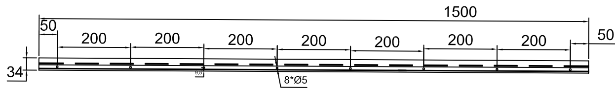
Front View
